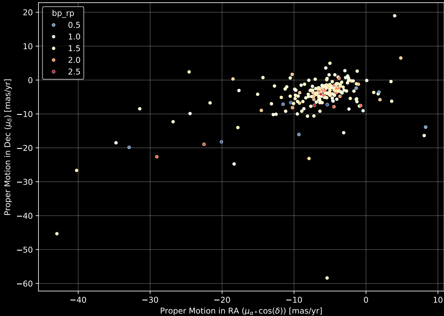
APOGEE DR17 Field: [311-12] Proper Motion Diagram (n= 210)
