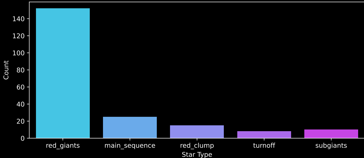
APOGEE DR17 Field: [311-12] Count plot of Star Type
