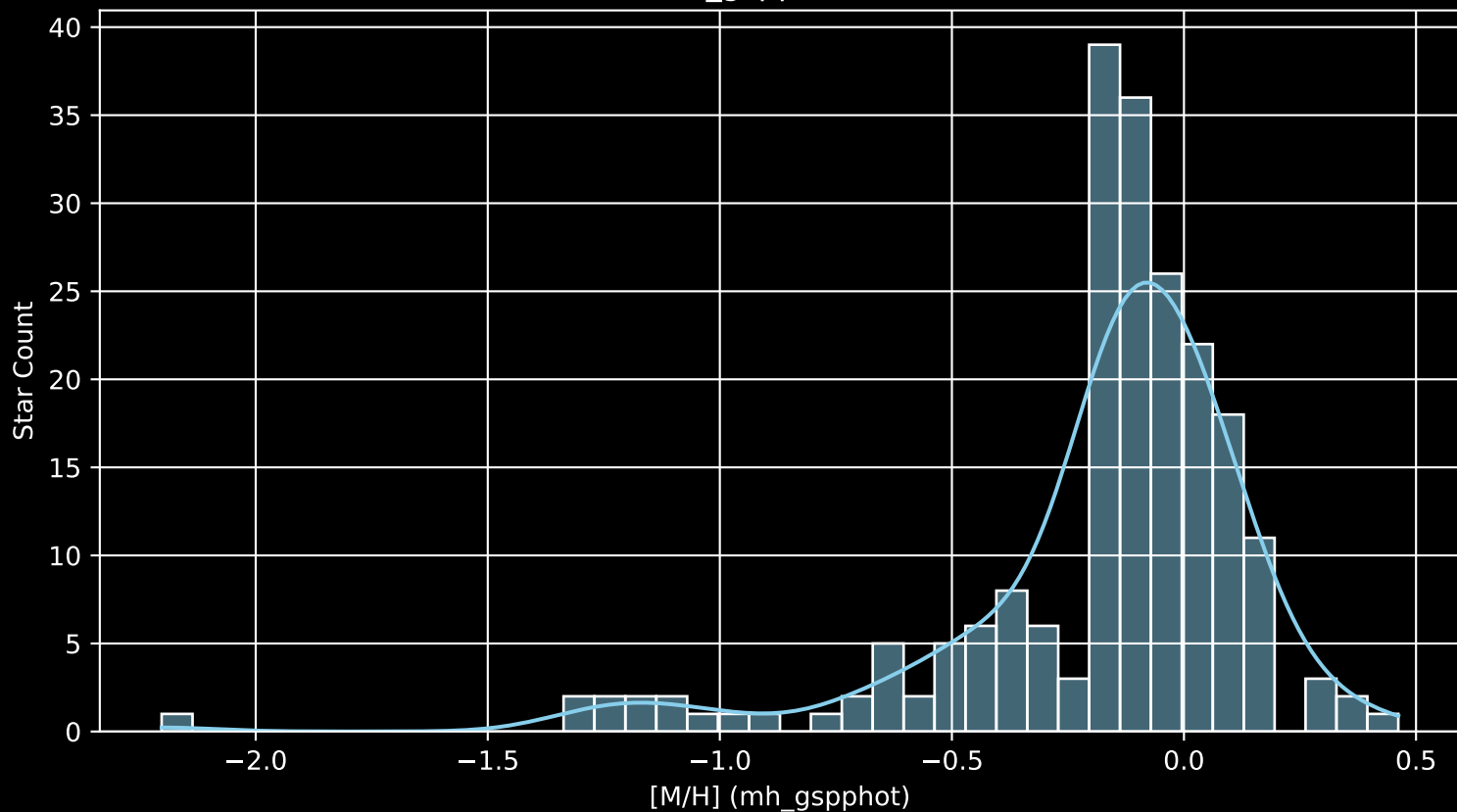
APOGEE DR17 Field: [311-12 [M/H] (mh_gspphot) (n= 208)
