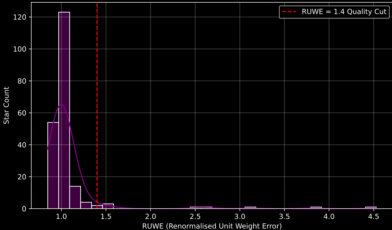
GAPOGEE DR17 Field [311-12] RUWE Distribution (n= 205)
