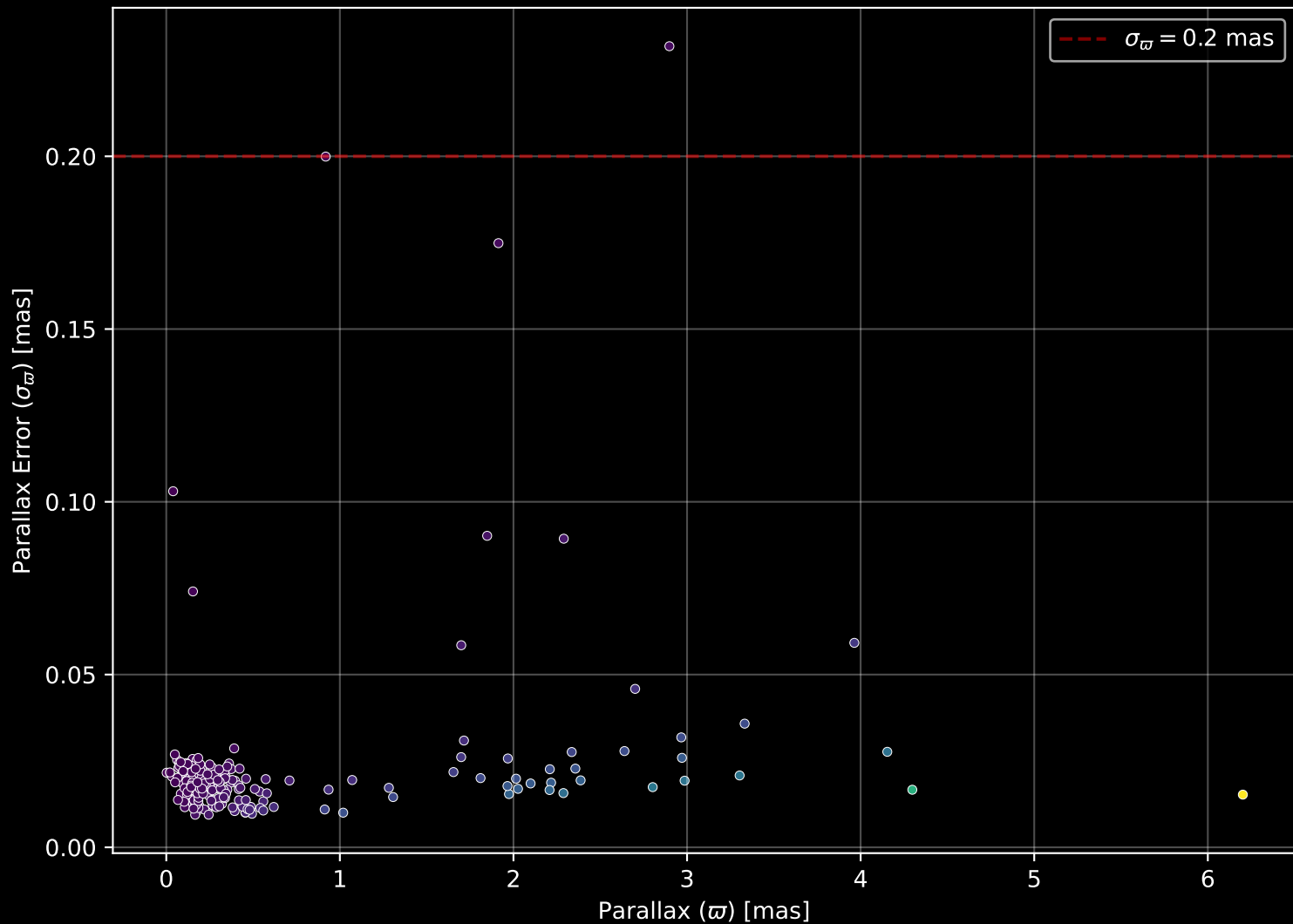
APOGEE DR17 Field: [311-12] Parallax Quality (n= 210)
